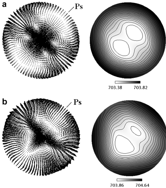
Fig. 5. Stationary three-dimensional flow in liquid bridge of As = 0.8 . (a) Velocity and temperature distributions on z = 0.5L observed at Ma = 44.90 ( m = 2 ). (b) Velocity and temperature distributions on z = 0.5L observed at Ma = 60.03 (mixture of m = 2 and m = 3 ). Temperature distributions are expressed by the gray scale.
