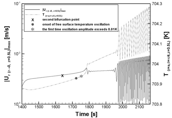
Fig. 7. Time evolution of three-dimensional oscillatory flow in liquid bridge of As = 0.8 , expressed by the indicator velocity ( |U_r(0, 0, 0.5L)|_{max} ) and a free surface temperature at (a, \pi/4, 0.5L) as a function of time.
