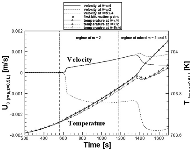
Fig. 6. Time evolutions of three-dimensional stationary flow in liquid bridge of As = 0.8 . Azimuthal velocities and temperatures observed at three different points at z = 0.5L are plotted as a function of time.
